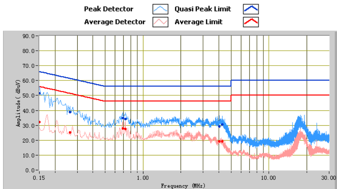
Phase Neutral Plot at 120Vac, 60Hz
